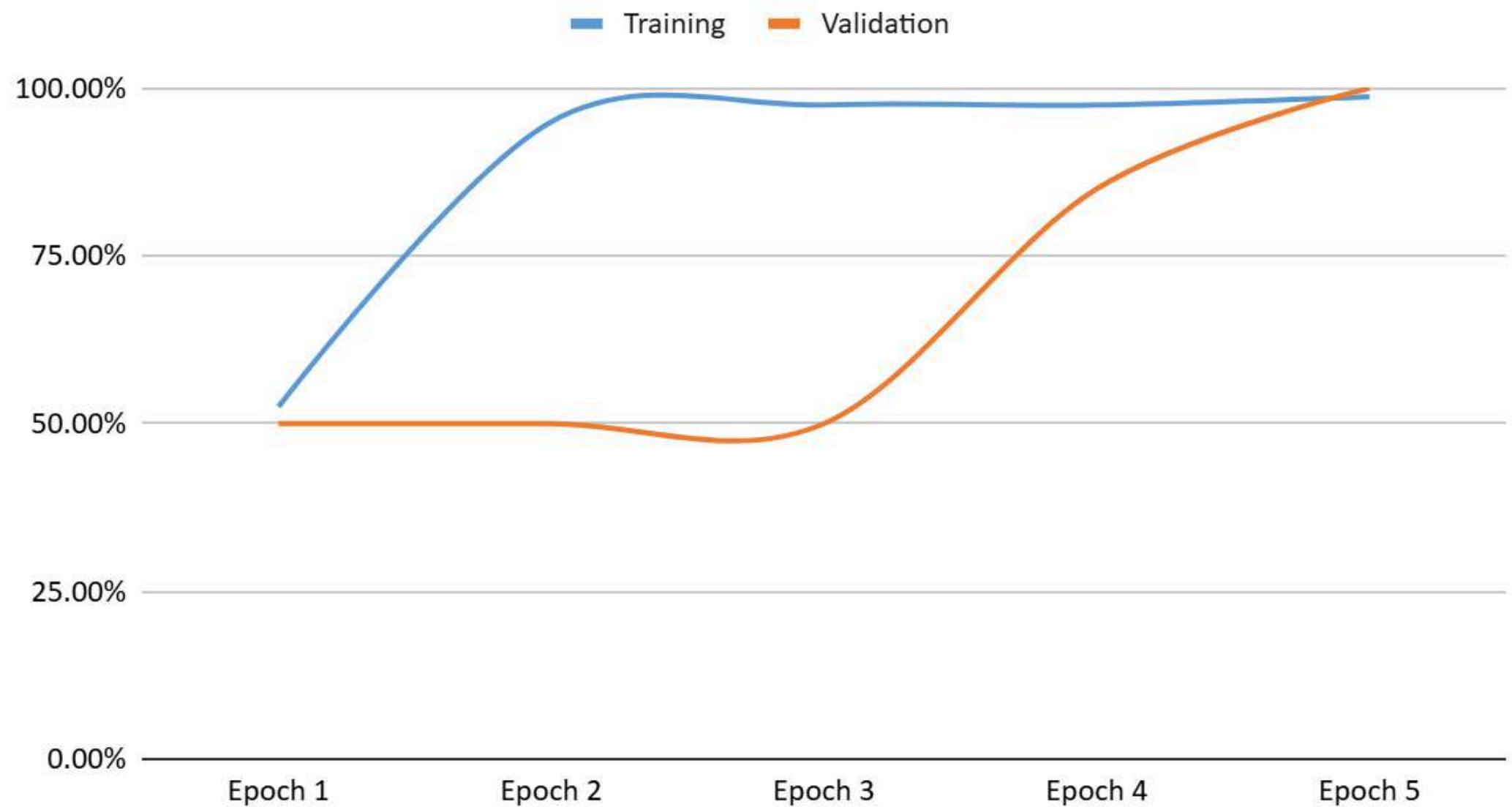
Akurasi Training VS Validation
